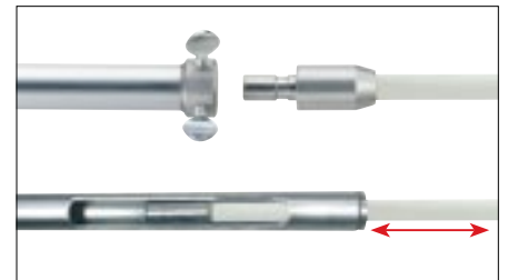
Fiberglass tip slides in and out of handle (cut-away view)
