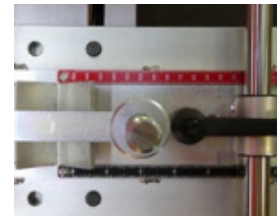
Front roller 'V' brackets with new positioning scales
